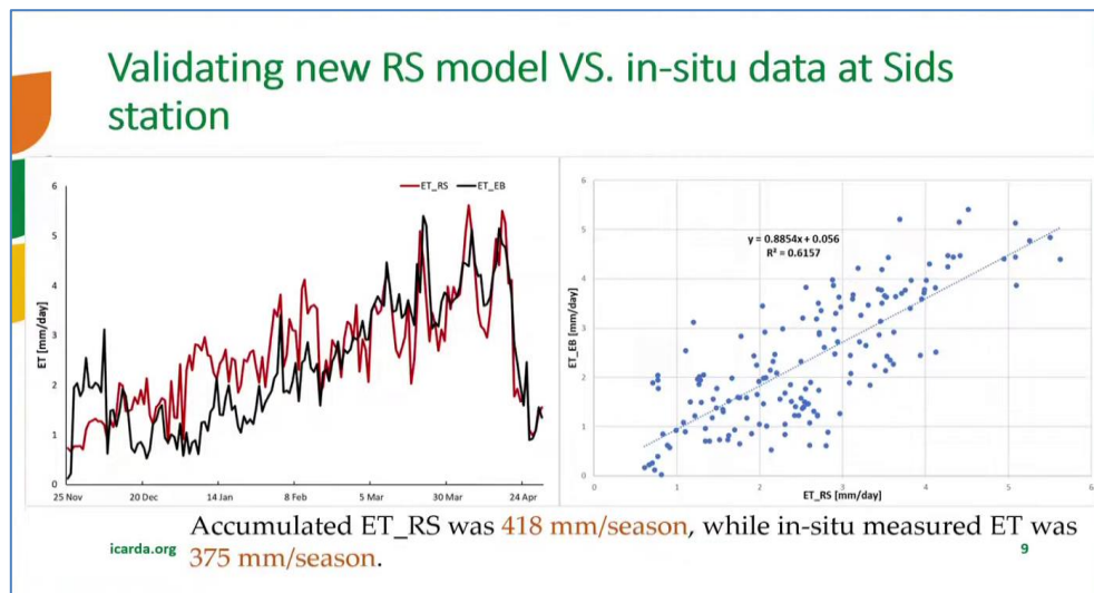
Validating new RS model VS. in-situ data at Sids station.
